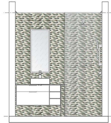
ELEVATION H
